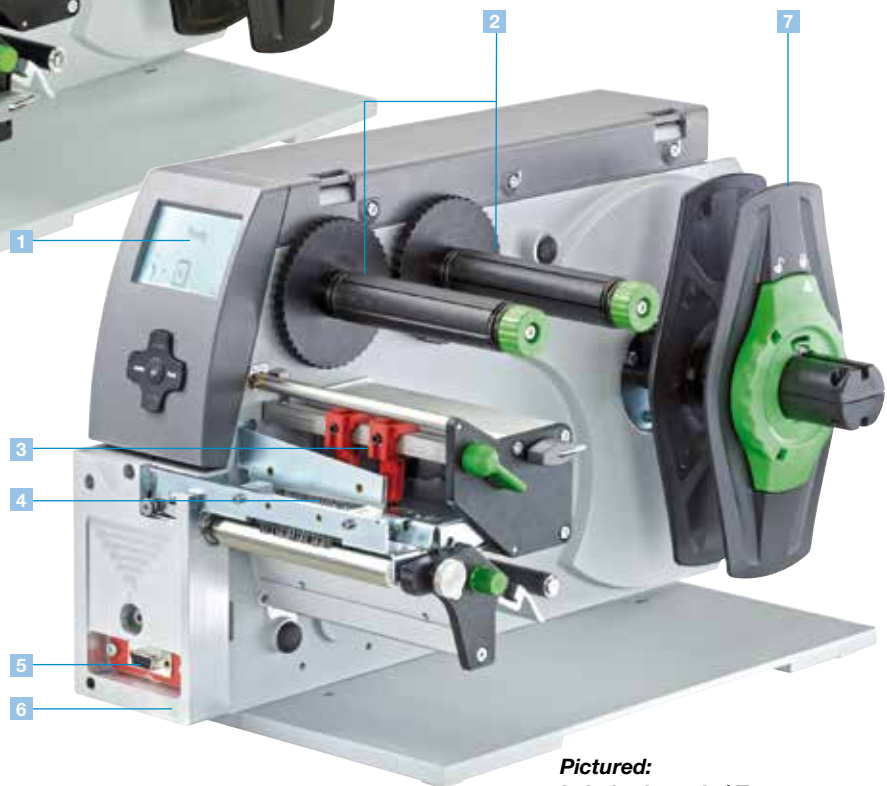
Pictured: Label printer A4+M with centered material positioning
